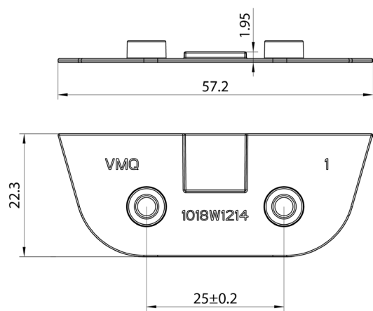
Rubber pad dimensions (mm)
