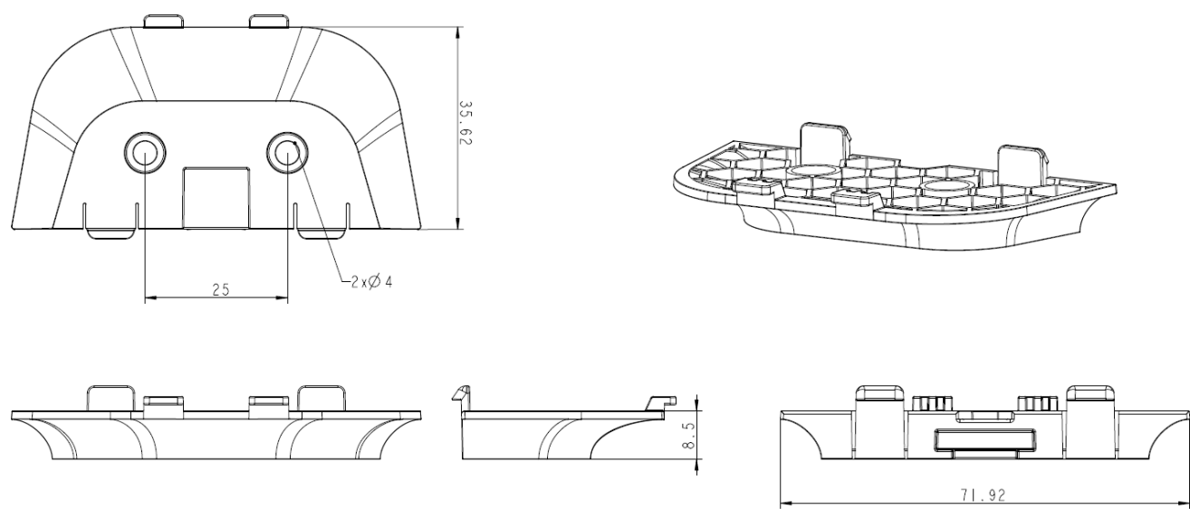
Flat mount dimensions (mm)
